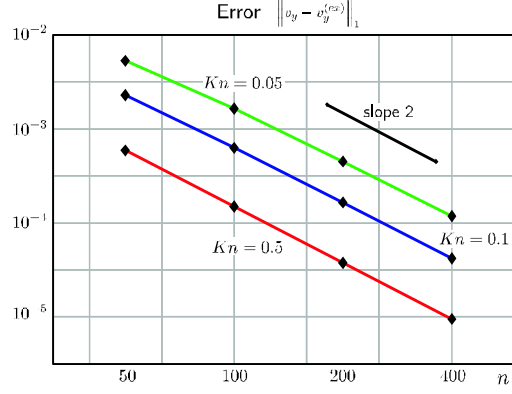
Figure 3: Empirical convergence of the proposed numerical method. Velocity of the linear R13 equations compared with exact solution for different grids and Knudsen numbers.
